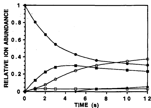
Figure 1. Time dependence of the relative abundances of the charged species following introduction of ions 1 into a 30:1 H_2O/CH_3OH gaseous mixture at 298 K and a total pressure of 2.1 \times 10^{-7} Torr: (●) 1; (■) 2; (○) CH_3OH_2^+ ; (□) NO_2^+ ; (◆) (CH_3)_2OH^+ .
