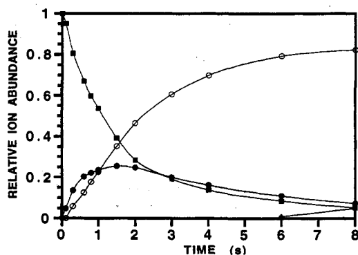
Figure 2. Time dependence of the relative abundances of the charged species following introduction of ions 2 into a 50:1 H_2O/CH_3OH gaseous mixture at 298 K and a total pressure of 2.6 \times 10^{-7} Torr. Labels are as in Figure 1.
